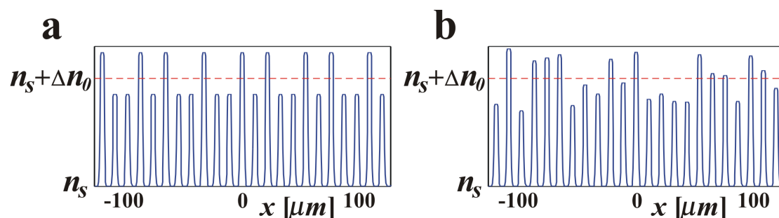
Figure 6.11: The refractive index profile of diagonal disordered Fibonacci and random lattice. a) Fibonacci lattice, b) random lattice.
