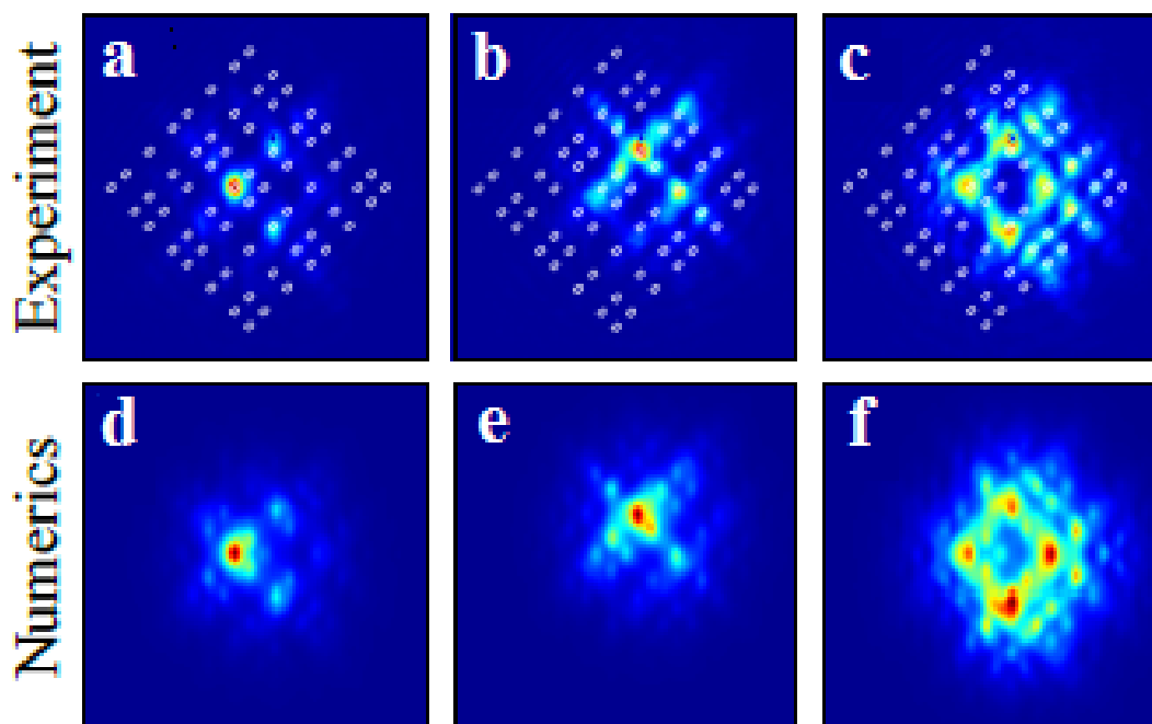
Figure 6.7: Light propagation through 2D Fibonacci lattice for three different input positions. Light intensity distributions at the exit face of the crystal. a-c Experimental results, d-f Numerical results.
